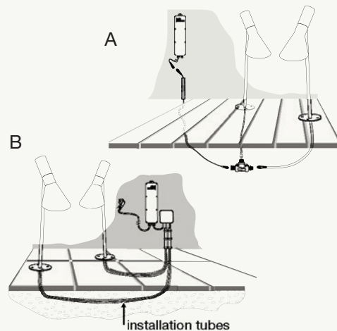
installation tubes
